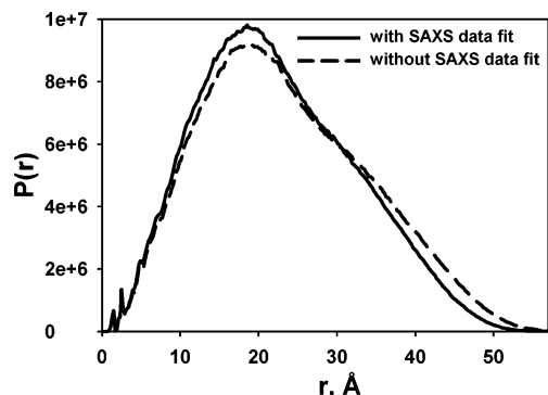
Figure 4. Impact of inclusion of SAXS data in the structure calculation on the distribution of the interatomic distances in the obtained structures. Each distribution is weighted by the products of the atomic numbers for each atom pair.
