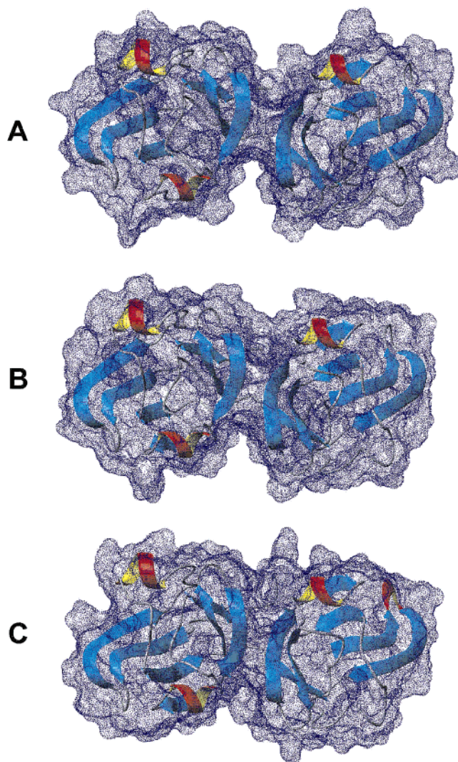
Figure 3. Impact of the SAXS data fit on the overall geometry. Protein backbones are shown in ribbon representation, and the molecular surfaces are calculated by sliding a 1.4-Å radius sphere over the molecule. (A) A representative model before SAXS data fit, (B) a representative model after SAXS data fit, and (C) the X-ray structure of \gamma B crystallin (1AMM) used to evaluate the accuracy of the atomic coordinates. The figure was generated using the program MOLMOL. 44
