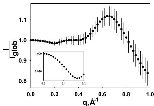
Figure 1. Globbic correction factor calculated as the ratio between the atomic and globbic scattering curves, I(q) and I_{\text{glob}}(q) , respectively. The mean and standard deviation of the curve points are calculated on the basis of 538 single-chain protein X-ray structures of 100–200 residues length, solved at resolutions of 1.8 Å or better. The calculations were carried out according to eqs 6 and 9. The inset shows the average correction factor calculated from the \gamma S crystallin models used in the final round of structure refinement.
